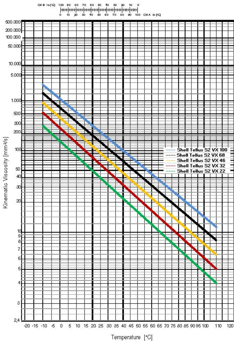
Viscosity - Temperature - Diagram
